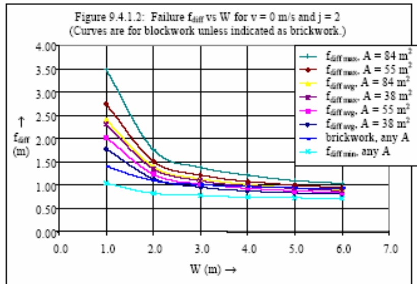
Figure 3 - Predicted Failure Curves for 2-storey Brick/Block Masonry Wall (Kelman 2002) ( F_{diff} = flood height difference outside to inside, W = wall width, A = floor area)
