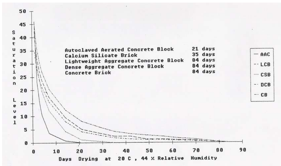
Figure 9 - Graph of Drying Times for Saturated Bricks & Blocks (H&H Celcon 2005)
