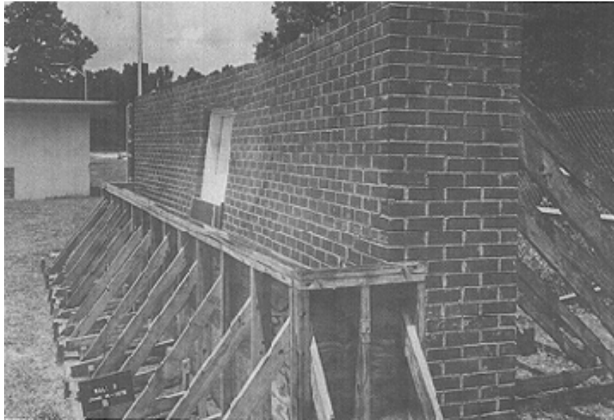
Figure 7 - Brick Wall Showing Failure after Hydrostatic Loading Test (USACE 1988)
