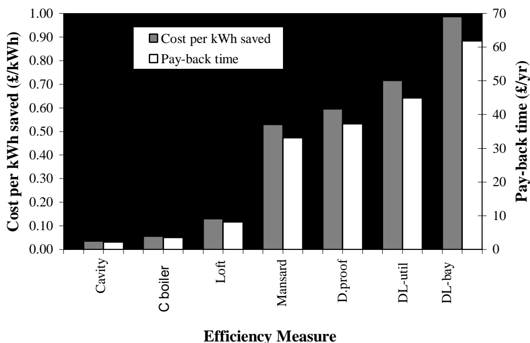
Figure 5 Cost effectiveness of individual measures in house type C 7
