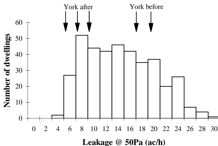
Figure 2 UK Pressurisation test data (after [14])
