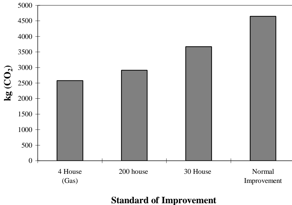
Figure 7 CO 2 emissions (measured gas consumption) - all schemes
